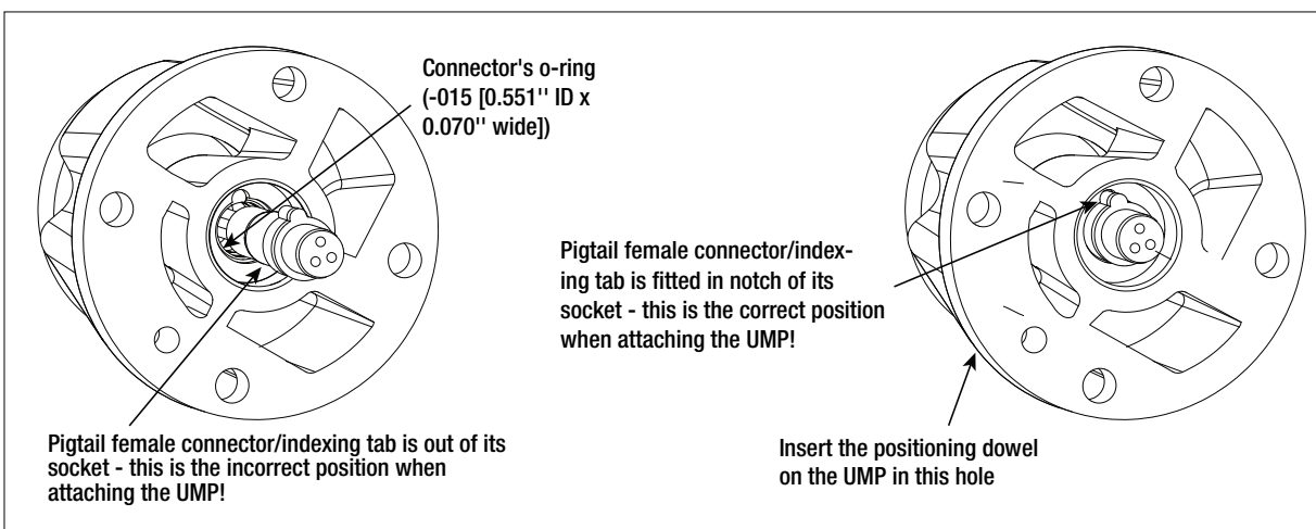
Figure 8. Verifying Pigtail's Female Connector Is Seated Properly
