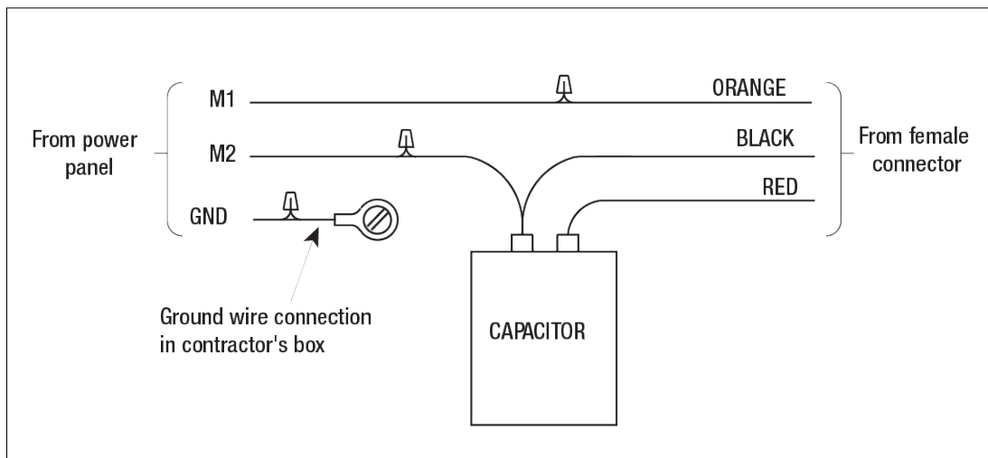
Figure 37. Wiring Schematic
