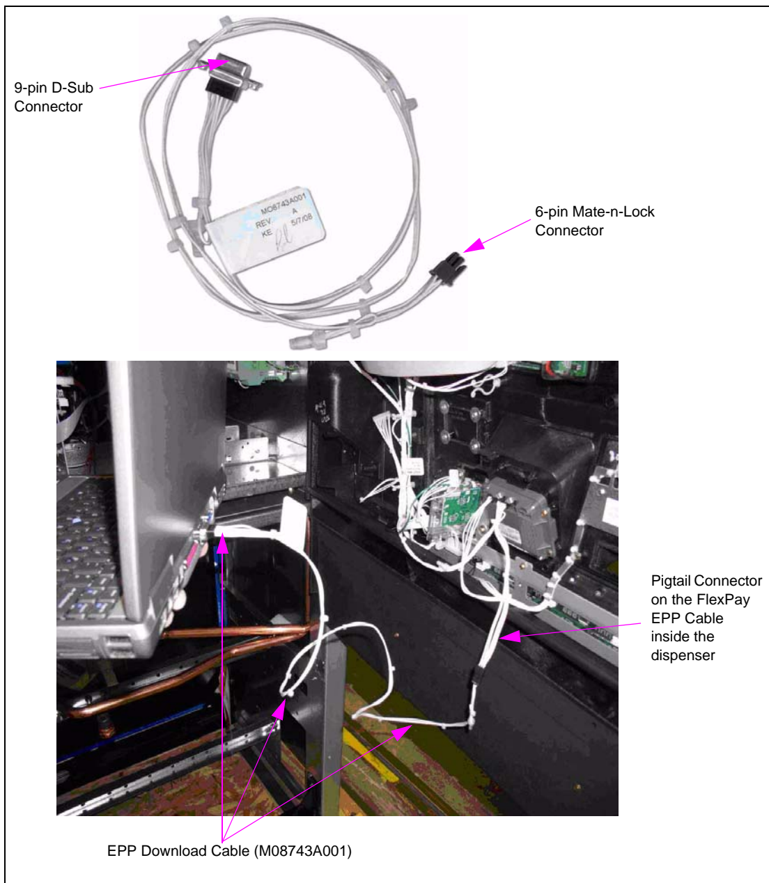
Figure 1: FlexPay EPP Download Cable (M08743A001)
