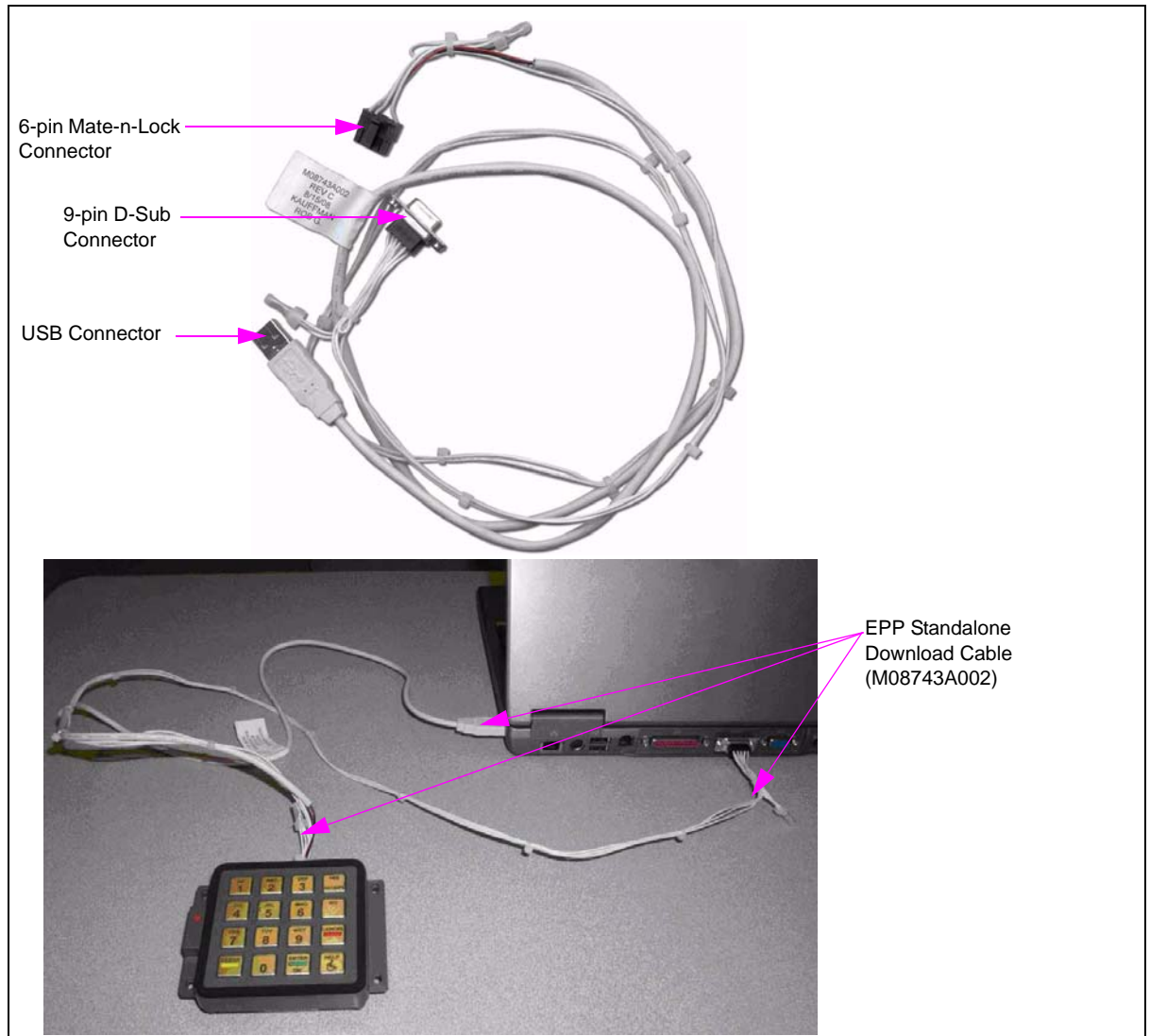
Figure 2: FlexPay EPP Standalone Download Cable (M08743A002)
