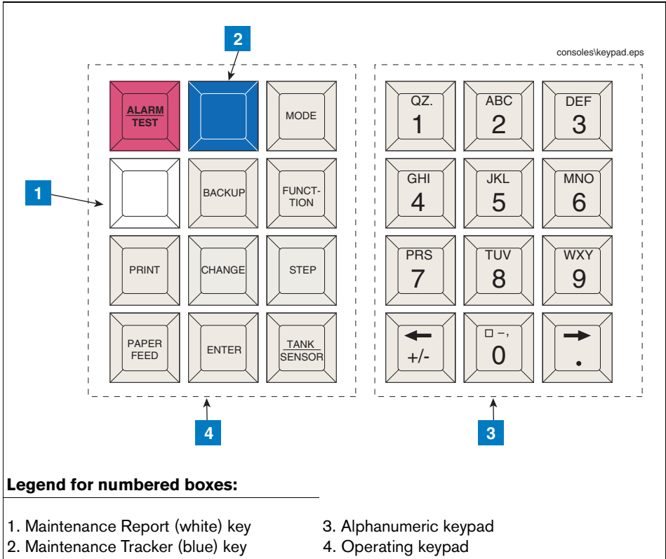
Figure 3-1. Console keypad
