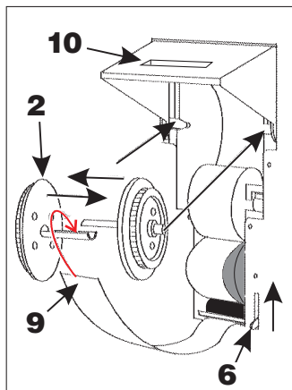
Figure 30-4.Paper change 4
