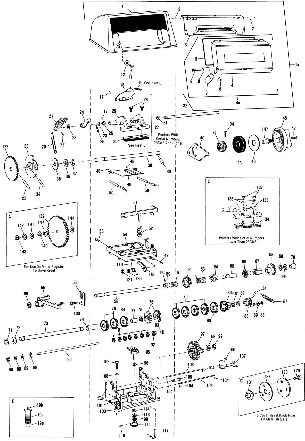
Meter Duplicator Direct Reading (Face Up) Zero Start (Reset) Type
