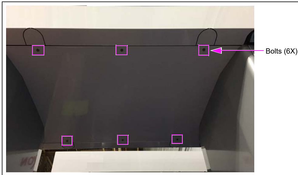
Figure 2: Removing Upper Housing Bottom Plate
