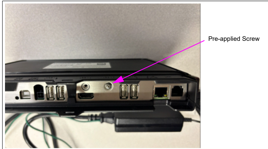
Figure 1: Removing the Pre-applied Screw
