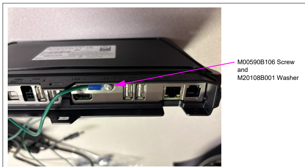
Figure 2: Ground Cable Attached
