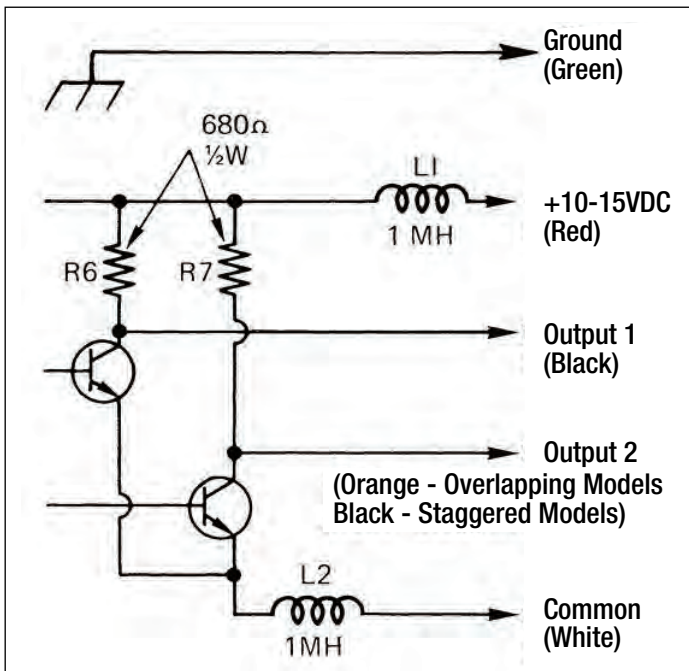
Figure 5. Wiring Connections for Dual Output Models
