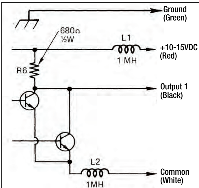
Figure 6. Wiring Connections for Single Output Models
