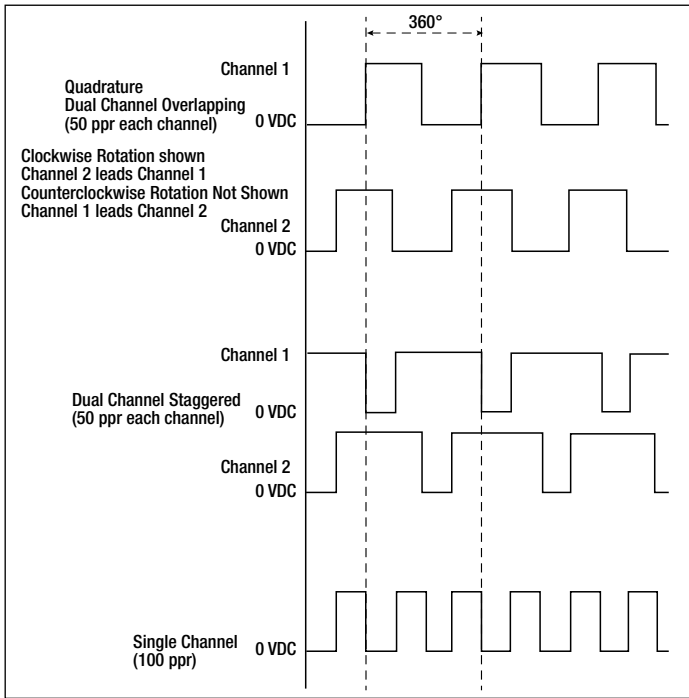
Figure 3. Logic Output Signals
