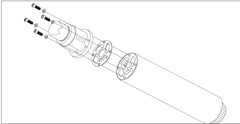
Figure 7. Aligning The UMP Gasket
