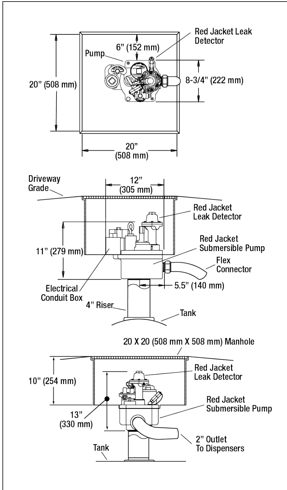
Figure 1. Leak Detector And Manifold Dimensions
