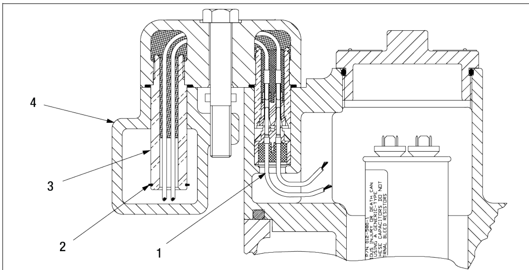
Figure 38. Yoke Assembly And Conduit Box Part Identification
