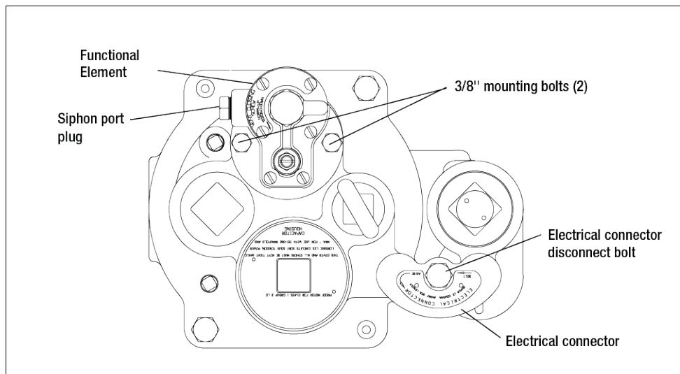
Figure 35. Packer With Functional Element
