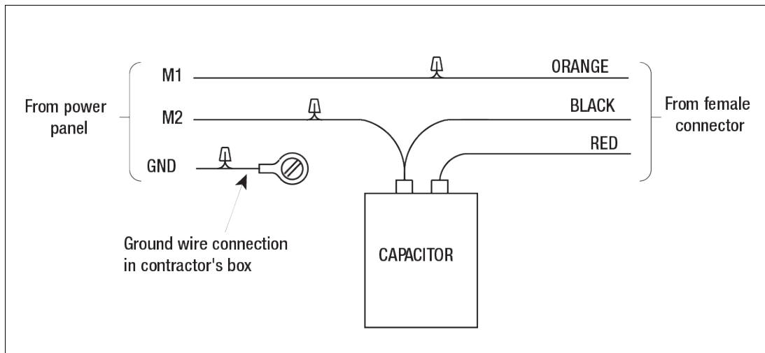
Figure 37. Wiring Schematic
