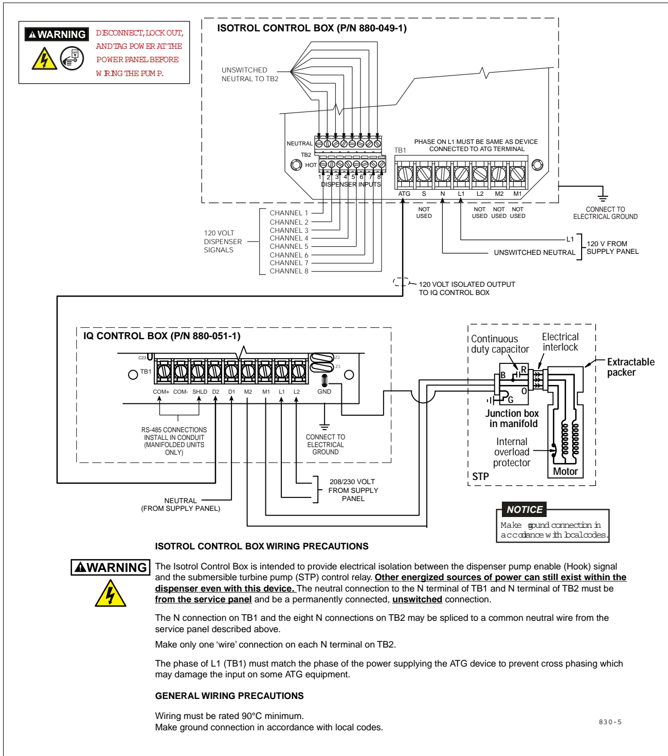
Figure 19. Isotrol To IQ System Wiring - 120 Volt Dispenser Signals
