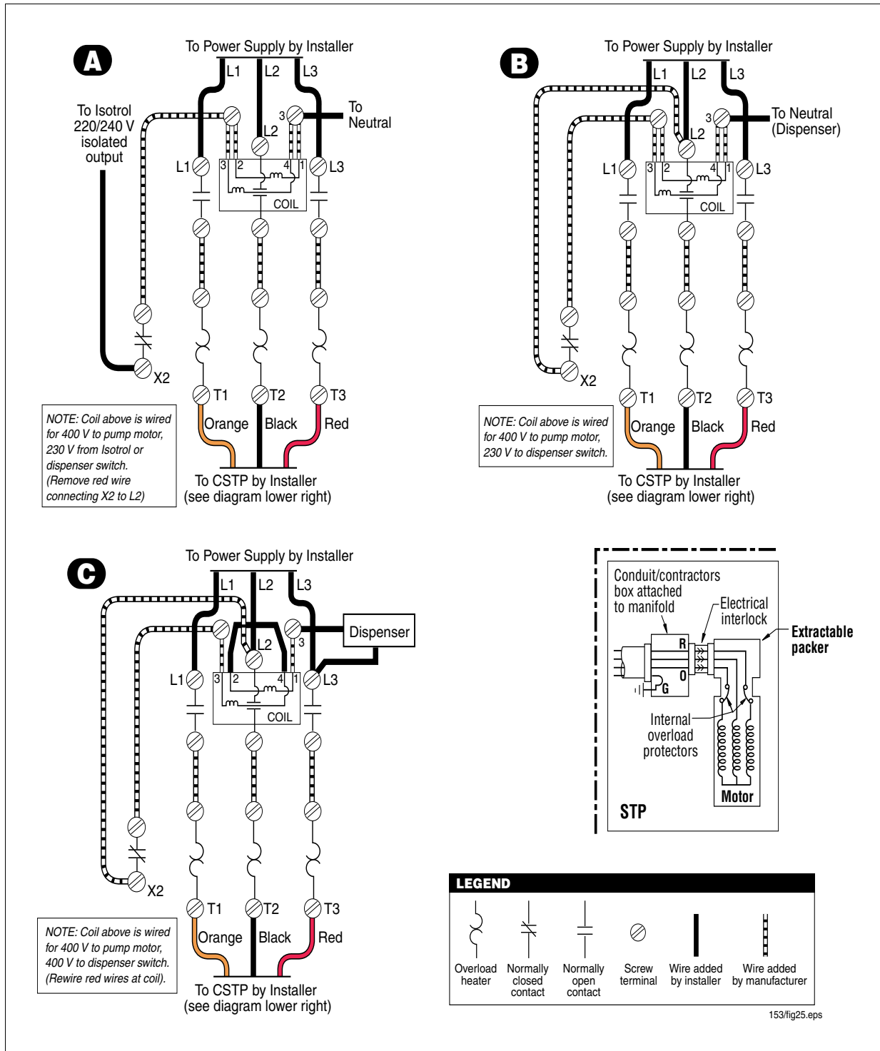
Figure 25. Three-Phase Pump Wiring Diagram Examples
