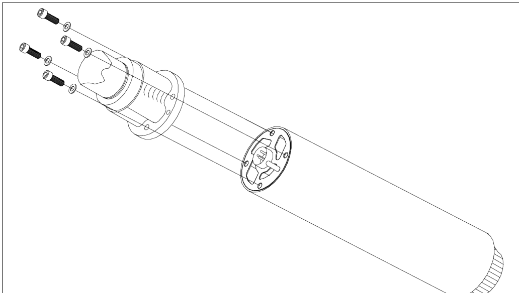
Figure 29. Removing The UMP
