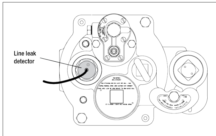
Figure 32. Electronic Line Leak Detector
