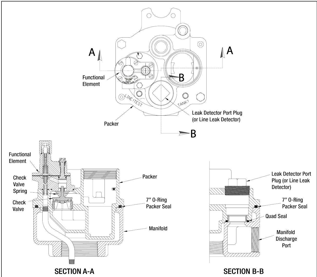
Figure 33. Locating 7" Packer O-Ring And Quad Seal
