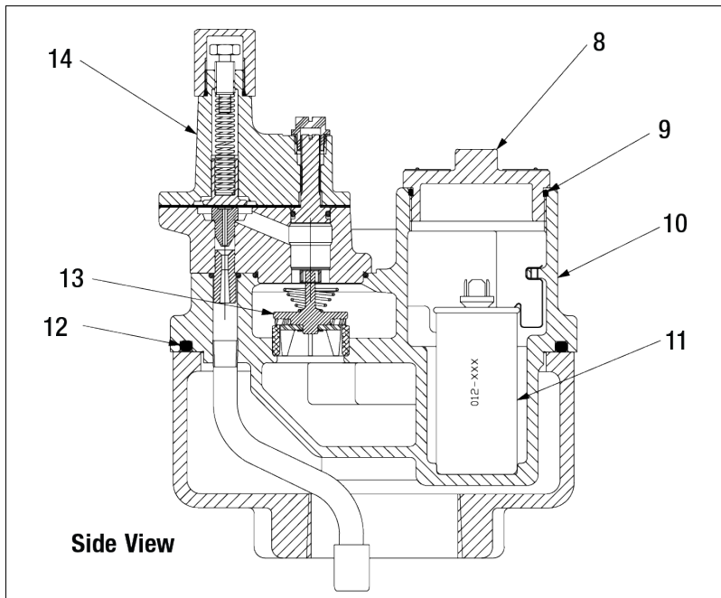
Figure 40. Packer-Manifold Assembly Side View- Part Identification
