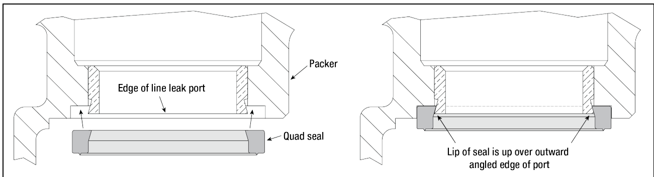
Figure 34. Installing New Quad Seal
