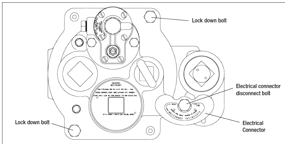
Figure 28. Packer
