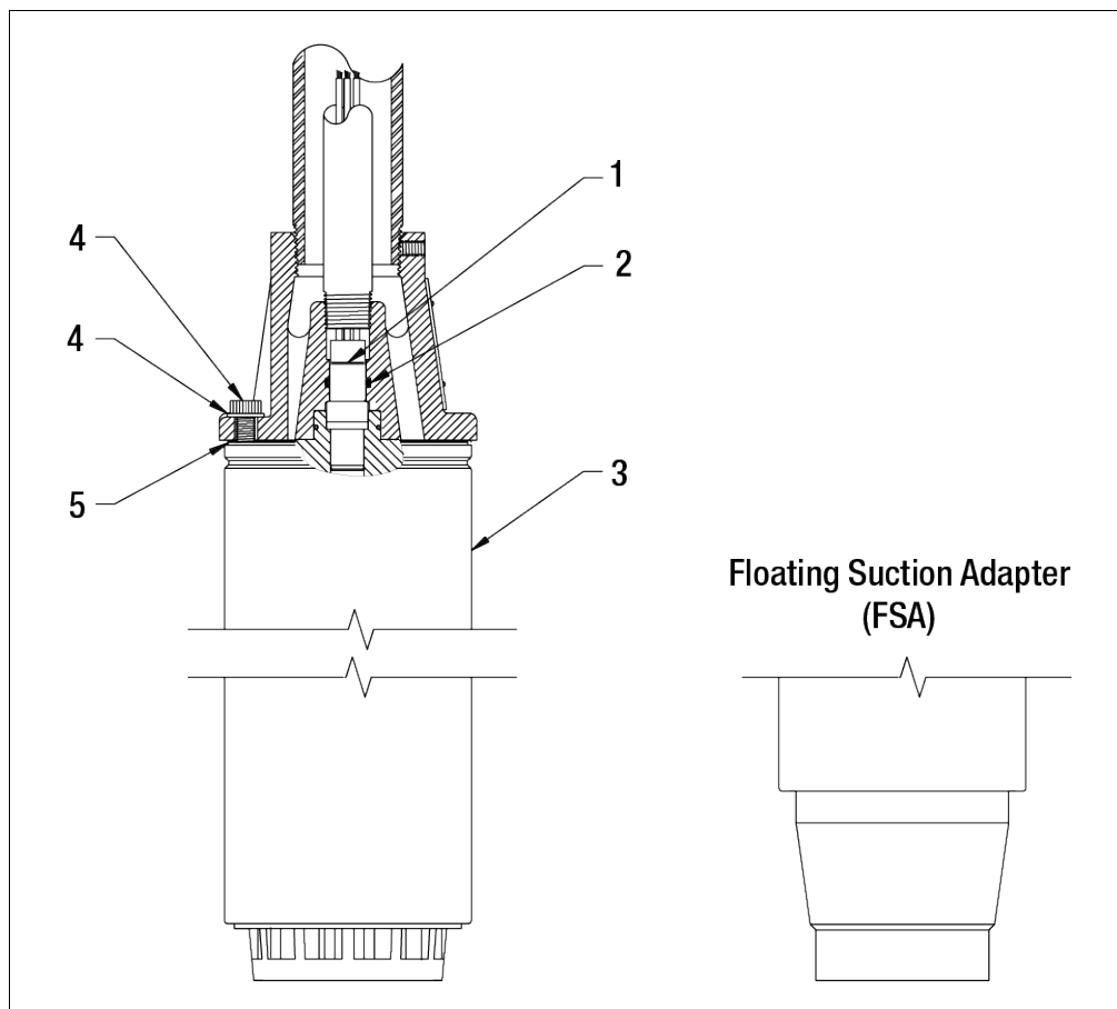
Figure 41. Pump Parts
