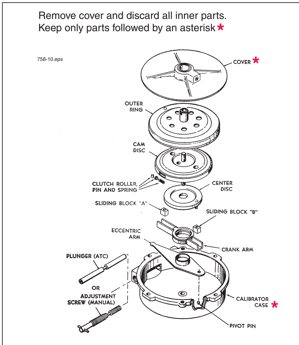
Figure 10. Disassembling The Smith Meter Calibrator
