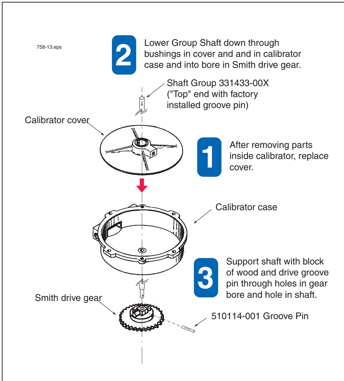
Figure 13. Reassembling The Smith Meter Calibrator
