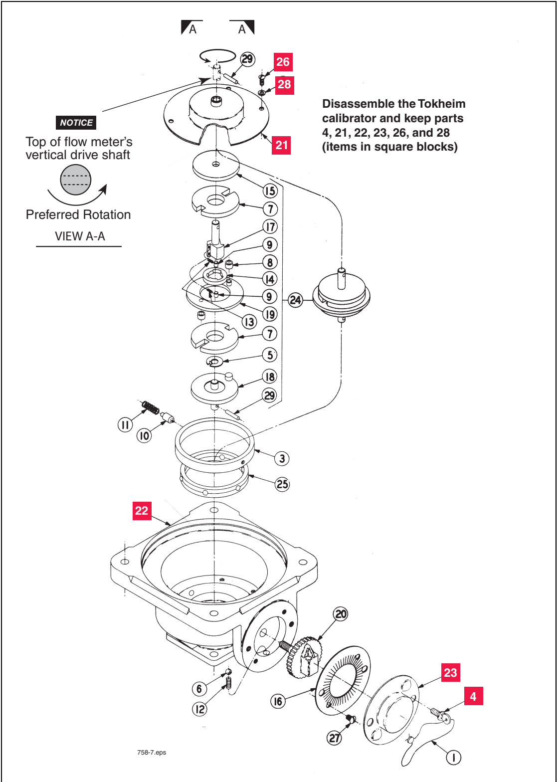
Figure 7. Disassembling The Tokheim Daniels, & Donovan Calibrator
