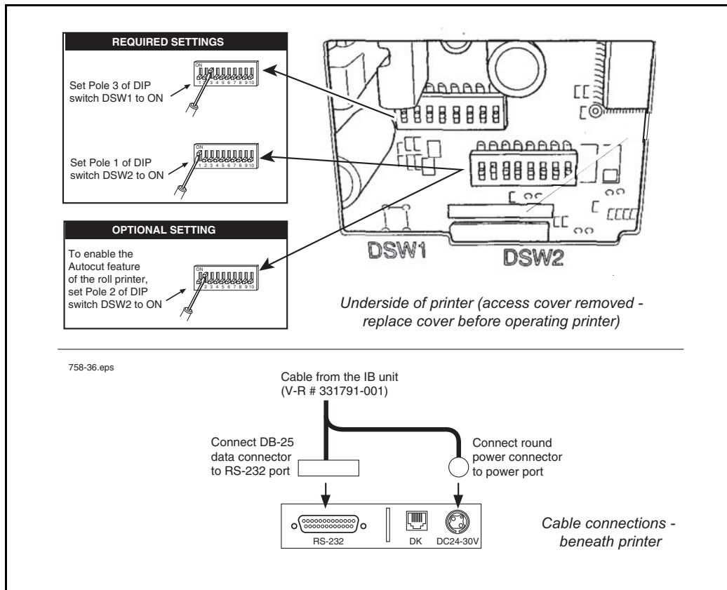
Figure 32. TM-U220A Roll Printer
