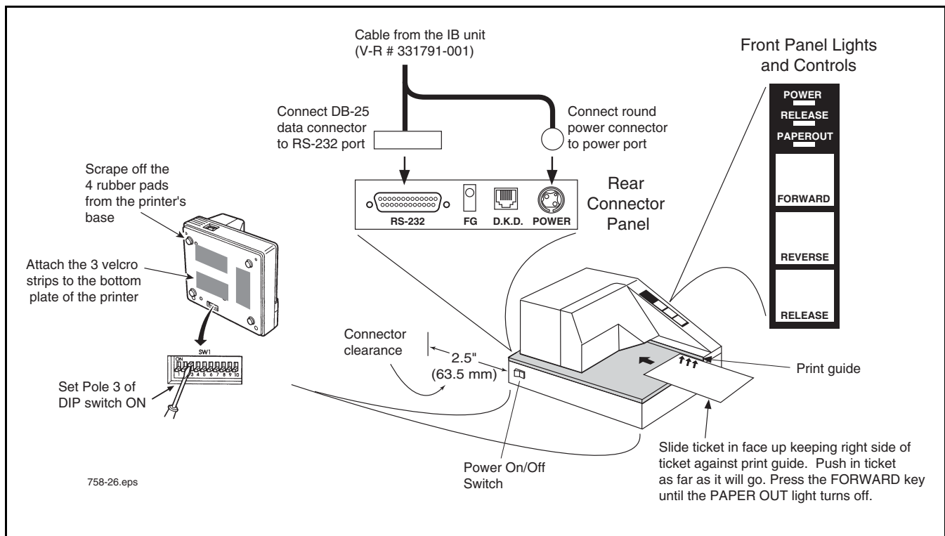
Figure 31. TM-U295 Printer
