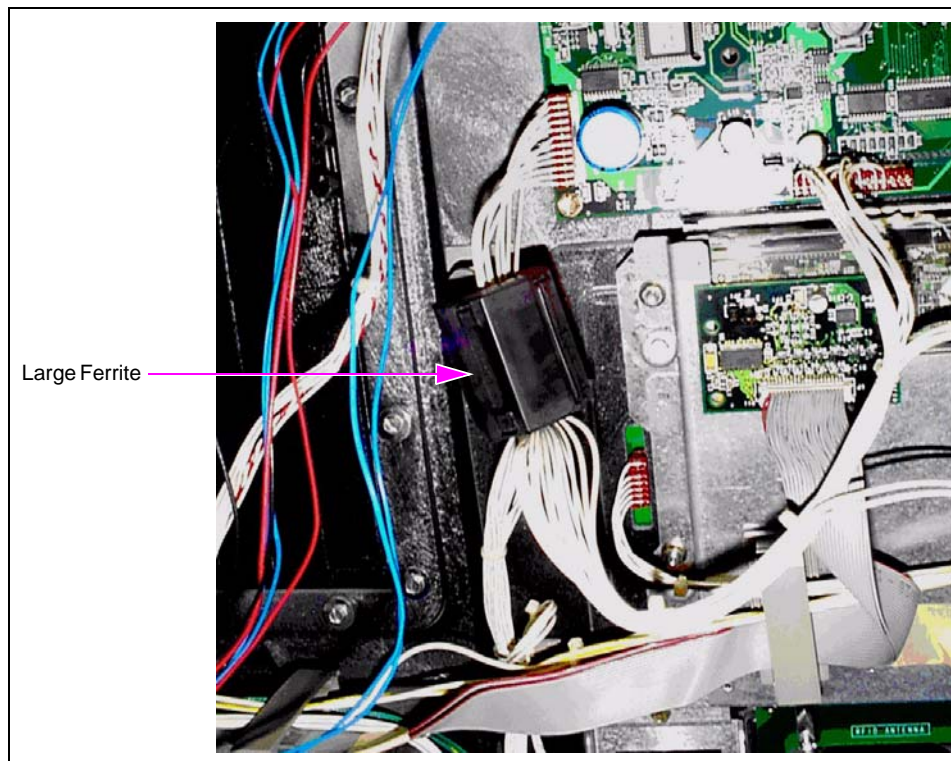
Figure 1: Installing the Large Ferrite on the Door Node Cable
