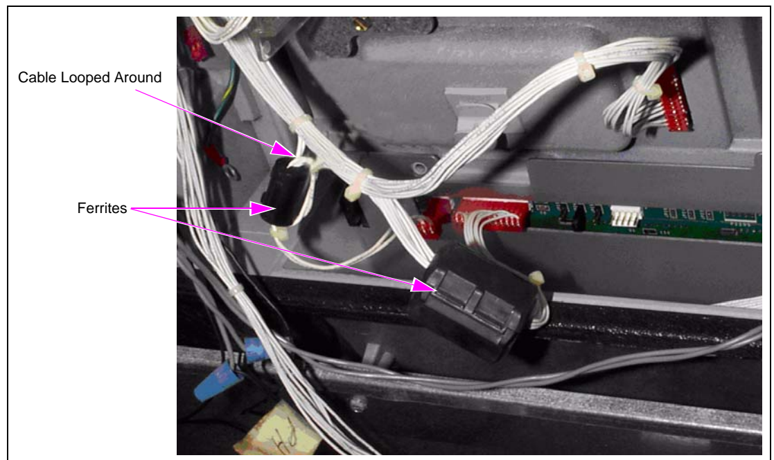
Figure 2: Installing the Two Ferrites on the Cables at the PPU Board
