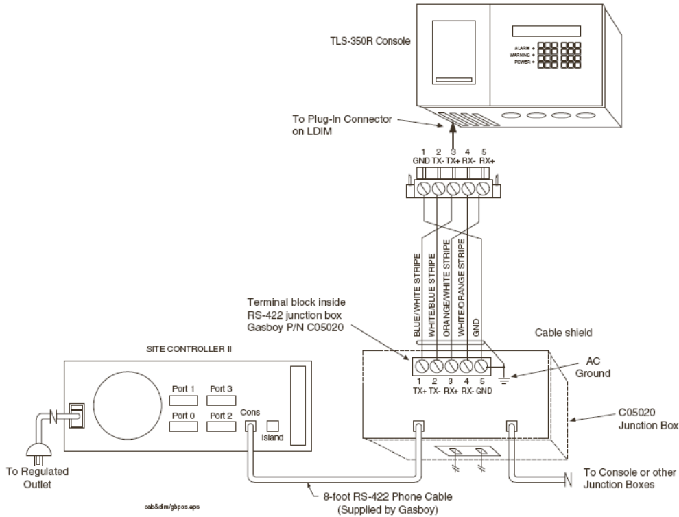
Figure 20. Gasboy Console Loop Connection
