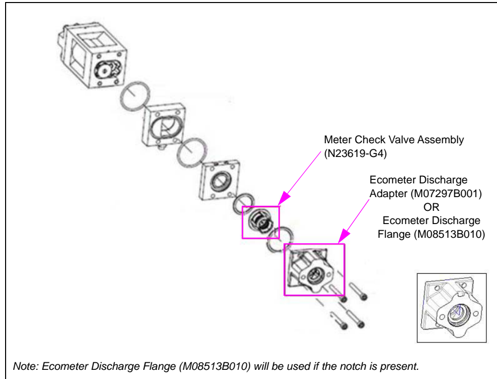
Figure 4: Assembling Check Valve
