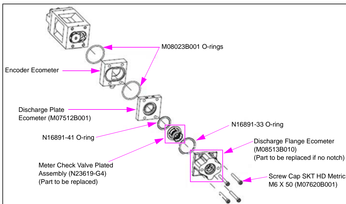
Figure 3: Dismantling Meter Assembly
