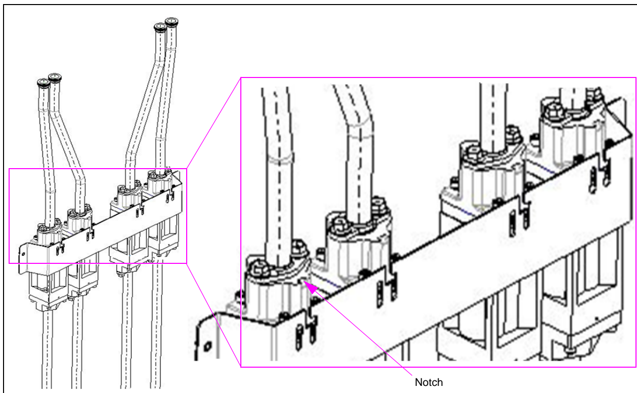
Figure 3: Dismantling Meter Assembly
