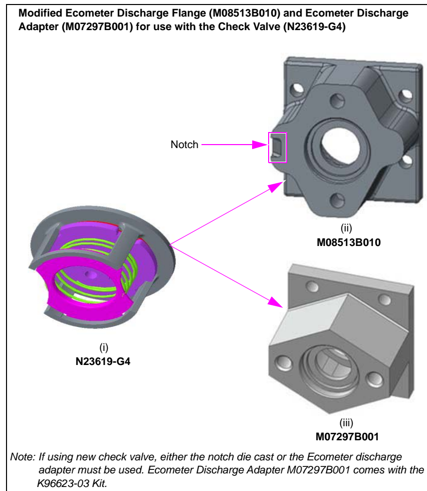
Figure 1: Modified Ecometer Discharge Flange (M08513B010) and Ecometer Discharge Adapter (M07297B001)
