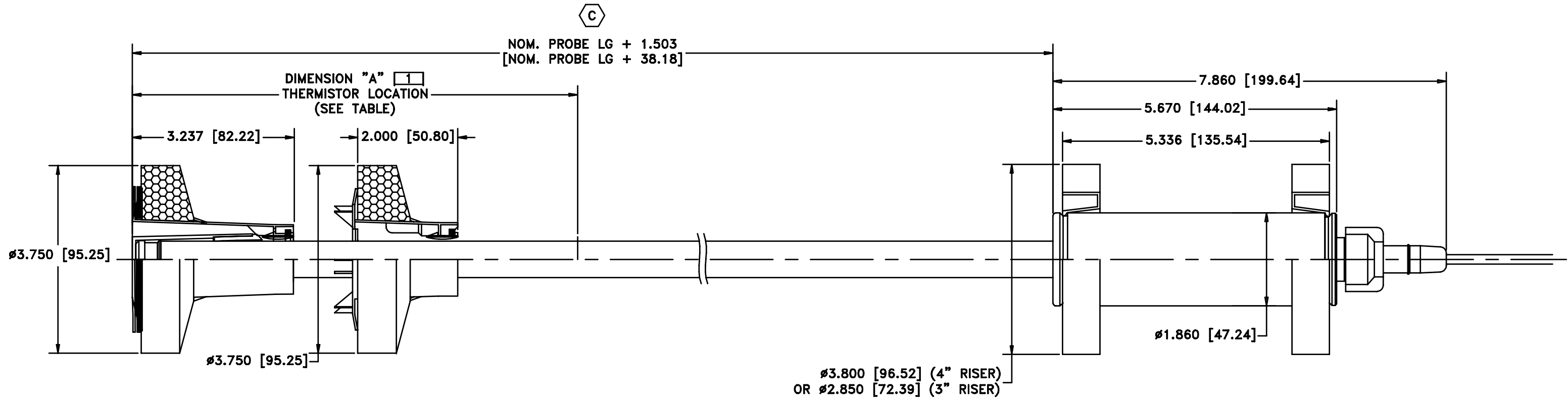
VIEW SHOWN WITH 4" FLOATS
