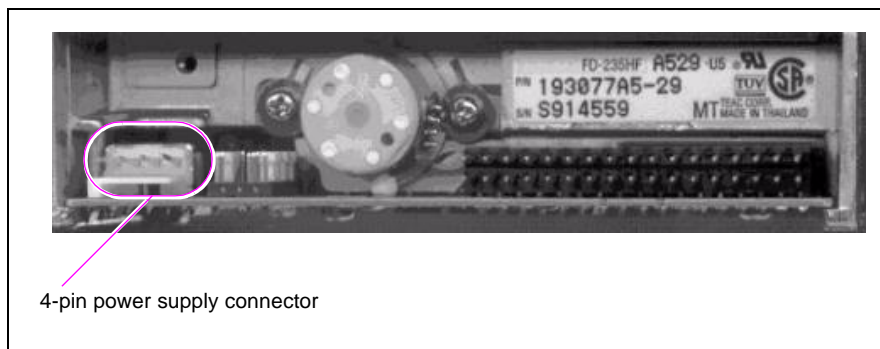
Figure 1: Location of 4-pin Power Supply Connector on Floppy Disk Drive
