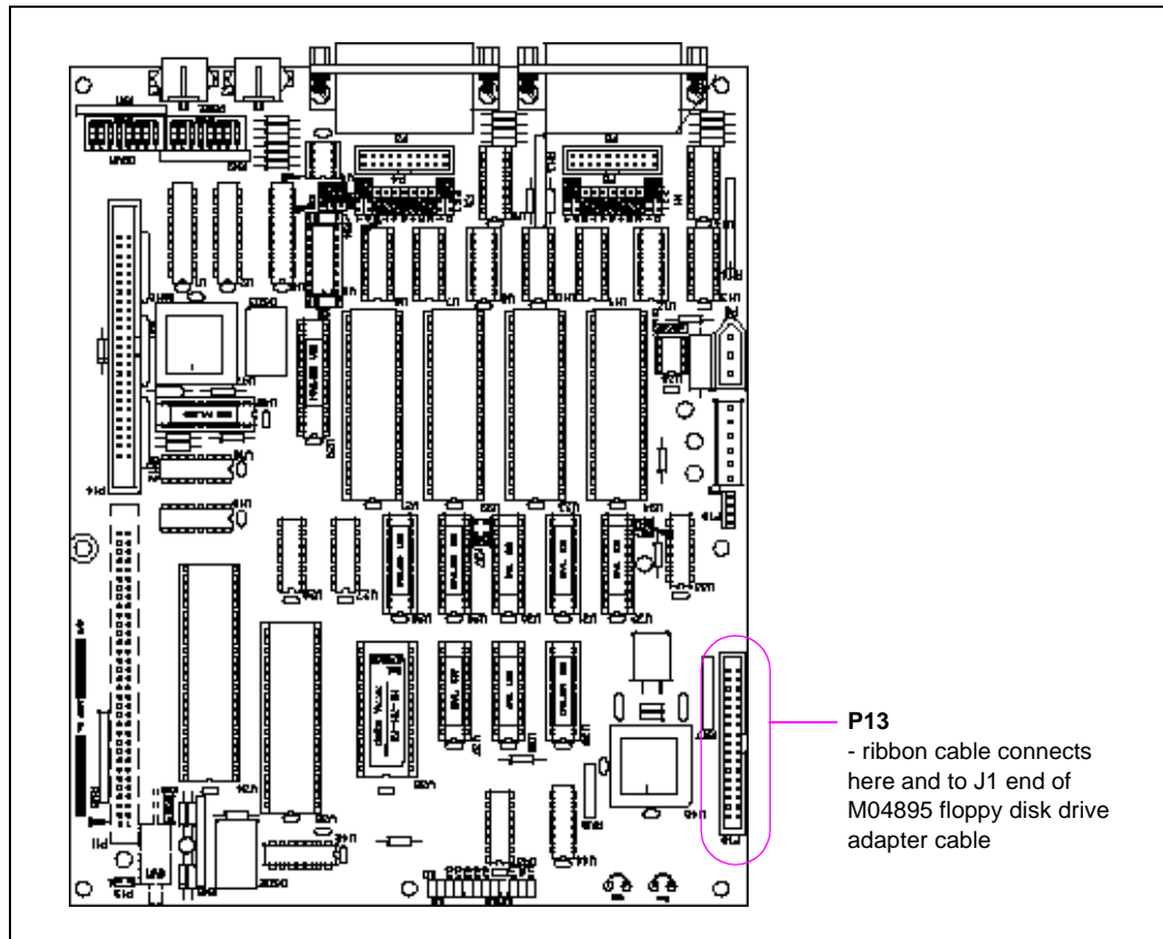
Figure 4: Location of P13 on Site Controller II CPU PCB
