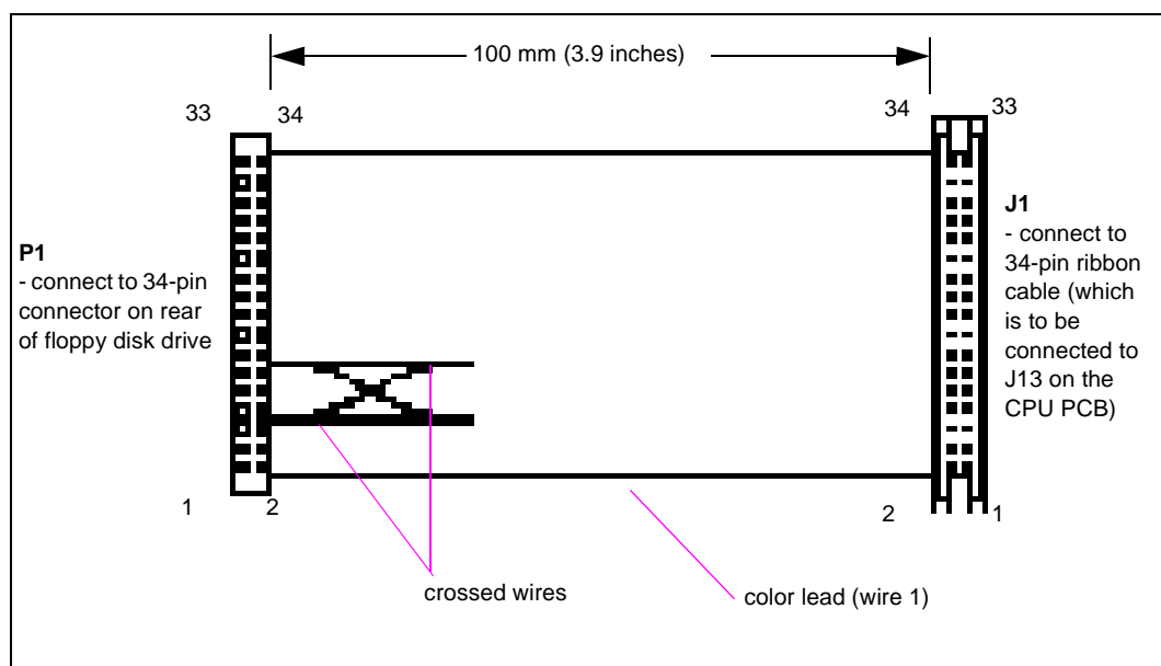
Figure 2: M04895 Floppy Disk Drive Adapter (Ribbon) Cable
