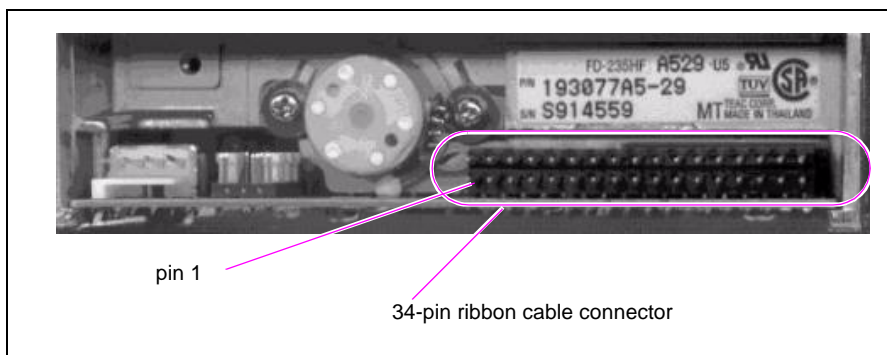
Figure 3: Location of 34-pin Ribbon Cable Connector on Floppy Disk Drive
